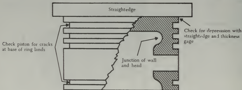
FIGURE 10-6. Checking a piston head for flatness.
